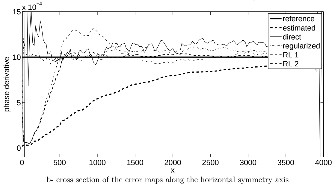
Figure 6: Comparison of the results obtained with various deconvolution techniques. No noise
