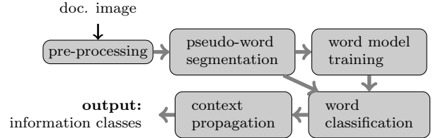
Figure 1. Work-flow showing several consecutive stages, starting from pre-processing to output i.e., \mathcal{H\&P} text separation.
