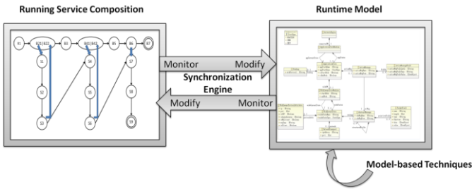
Figure 4 Approach Architecture
