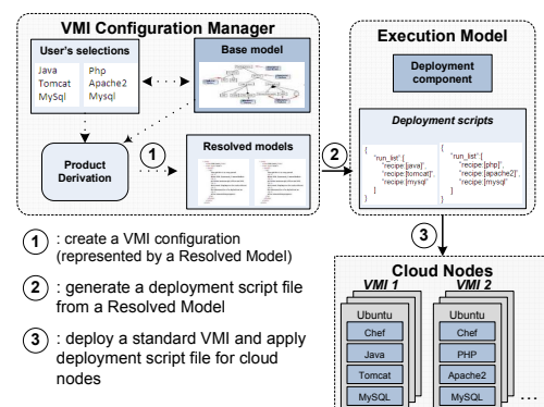
Figure 4. Model-Driven Deployment Process
