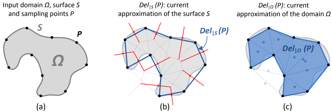
Figure 3: (a) Input domain \Omega (gray area), boundary S (dark gray curve), and points P (black dots) sampling the surface. (b) Del_{|S}(P) , the Delaunay triangulation restricted to surface S , is formed by edges (thick blue segments) whose dual Voronoi edges (thick red segments) intersect S . (c) Del_{|\Omega}(P) , the Delaunay triangulation restricted to the domain \Omega , is formed by triangles (in blue) whose circumcenters (blue dots) lie inside \Omega .
