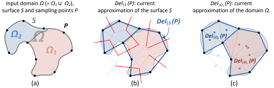
Figure 4: (a) Input domain \Omega = \Omega_1 \cup \Omega_2 (pink and light blue areas), boundary S (dark gray curve), and points P (black dots) sampling the surface. (b) Del_{|S}(P) , the Delaunay triangulation restricted to surface S , is formed by edges (thick blue segments) whose dual Voronoi edges (thick red segments) intersect S . (c) Del_{|\Omega}(P) , the Delaunay triangulation restricted to the domain \Omega , is formed by triangles (in pink for \Omega_1 , in blue for \Omega_2 ) whose circumcenters (blue dots) lie inside \Omega .
