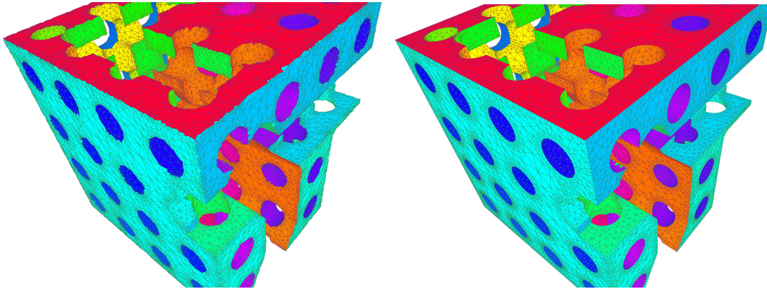
Figure 11: Cheese model. (left) Meshing without sharp features. (right) Meshing with sharp features. Input domain courtesy Distene.
