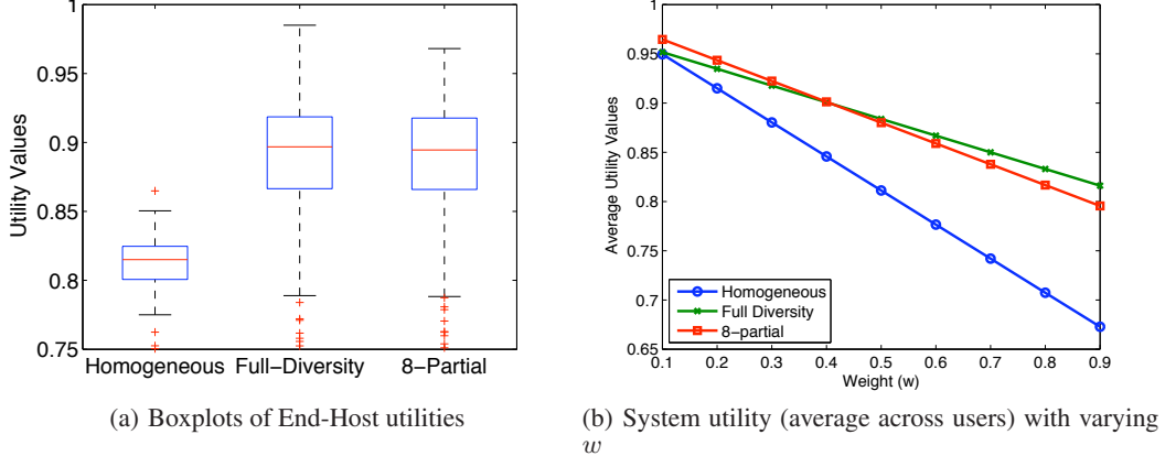
Figure 3: Comparison of Homogeneous, Full-Diversity, and Partial-Diversity policies
