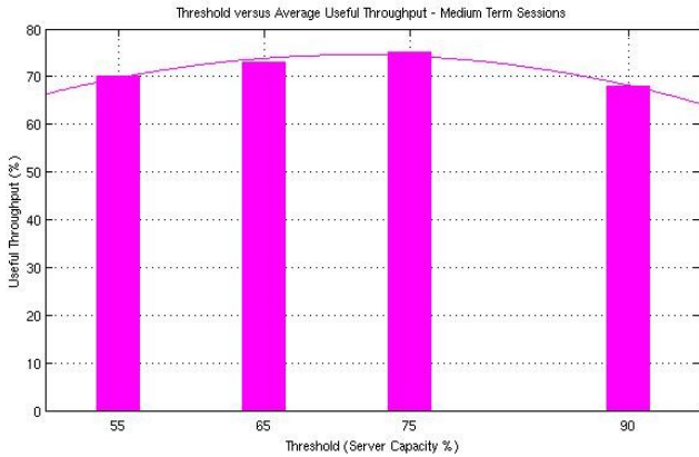
Fig. 3. Average Useful Throughput versus Threshold - Medium-Term Sessions & Responsive Session-Aware Admission Control.
