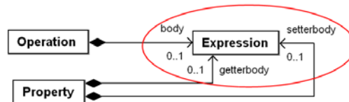
Fig. 3. Using operation bodies as join points between structure and behavior
