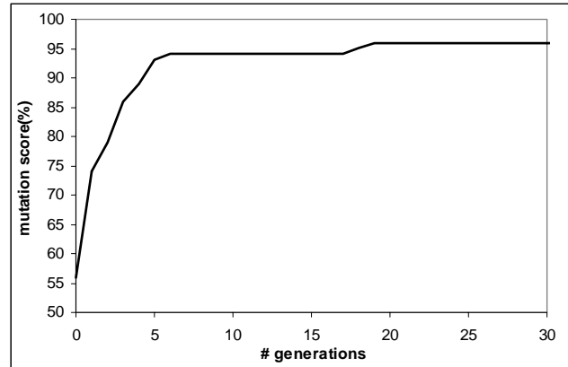
Figure 11 - Results of a bacteriological approach for system test data optimization
