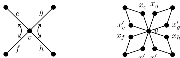
(a) v in G , T(v) = \{\{e, f\}, \{g, h\}\}
