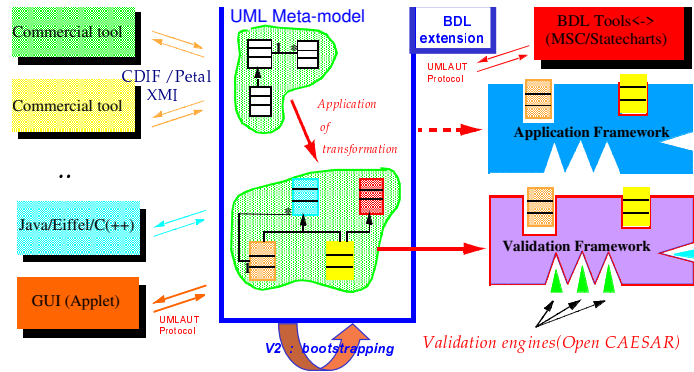
Fig. 2. UMLAUT Architecture
