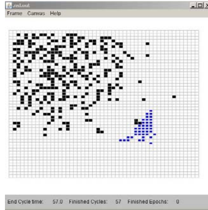
Fig. 1. Initial Configuration of the “aggregated” case.
