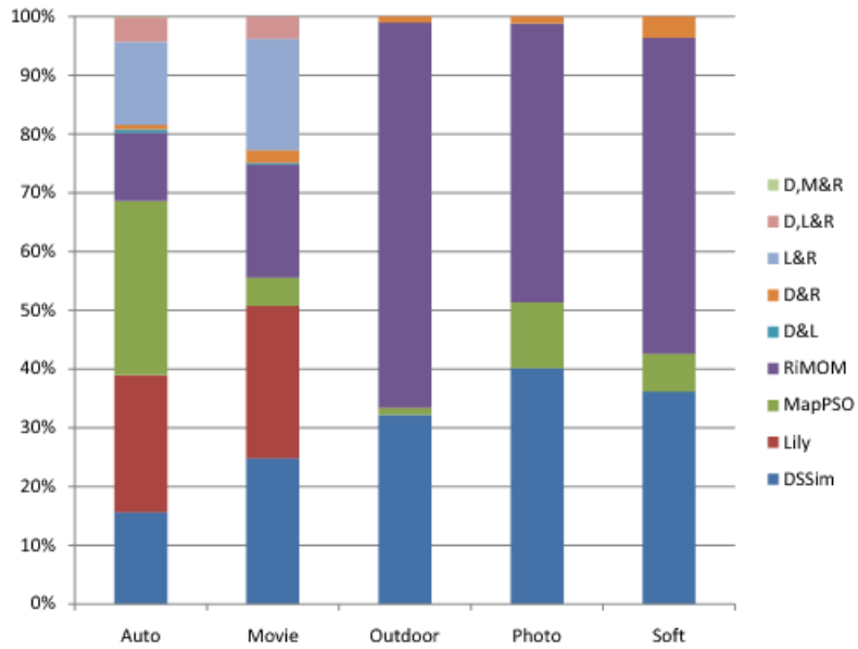
Fig. 10. Shared correspondences.
