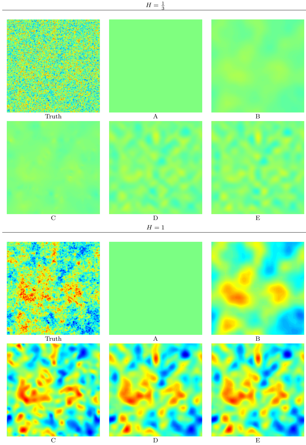
FIG. C.7. Estimated vorticity maps for methods A to E (see section 6.3 for a description) for H = \frac{1}{3} and H = 1 in the case of a very large regularization coefficient ( \sim 1e6 )
