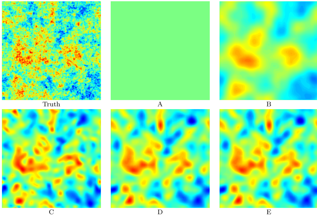
FIG. C.7. Estimated vorticity maps for methods A to E (see section 6.3 for a description) for H = \frac{1}{3} and H = 1 in the case of a very large regularization coefficient ( \sim 1e6 )
