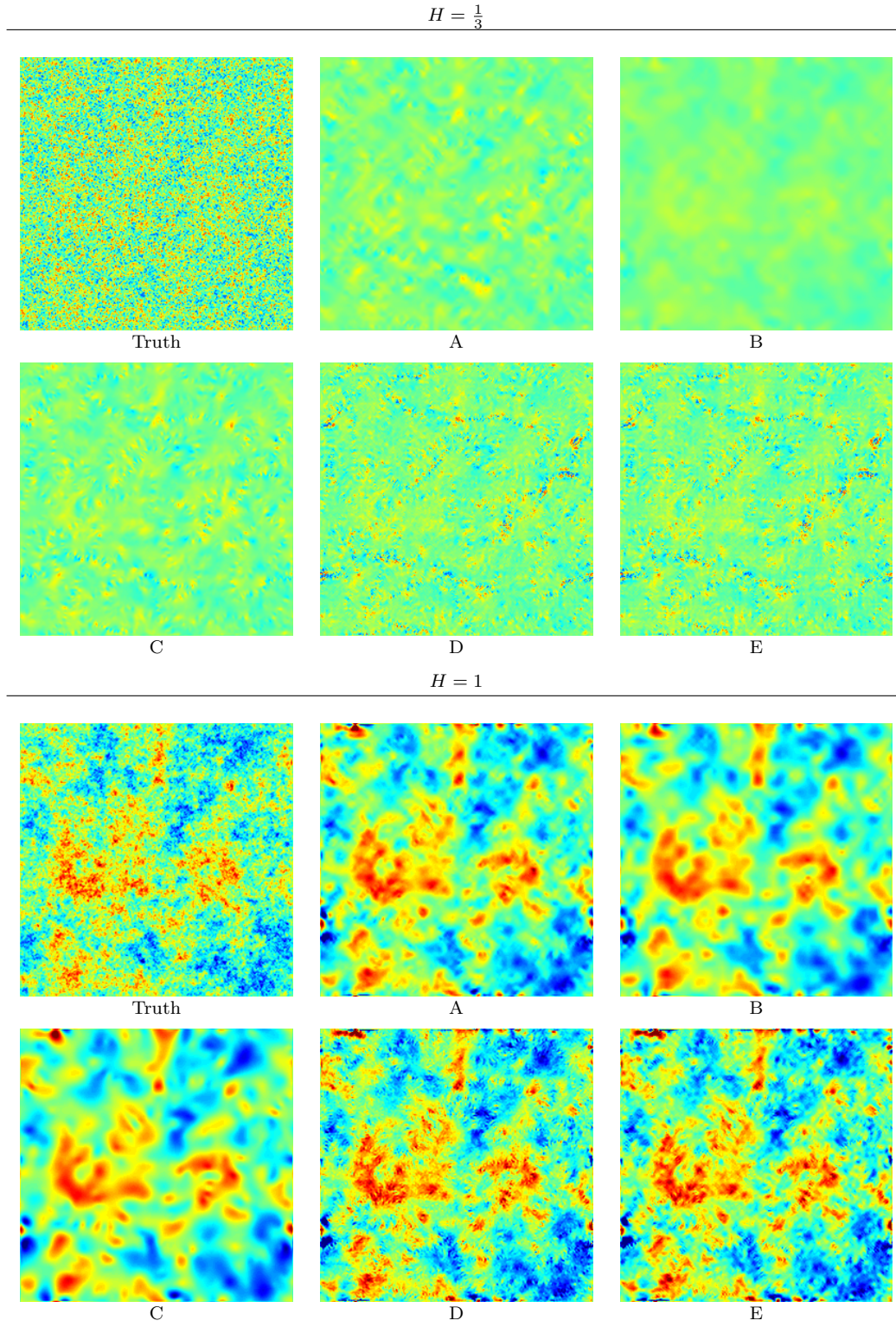
FIG. C.5. Estimated vorticity maps for methods A to E (see section 6.3 for a description) and for H = \frac{1}{3} (above) and H = 1 (below). Regularization coefficients were chosen to minimize the RMSE
