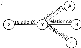
Fig. 1. N-ary relation
