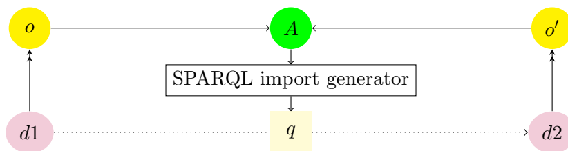
Figure 6.4: An import query can be generated from an alignment in order to import data from one data set into another.
