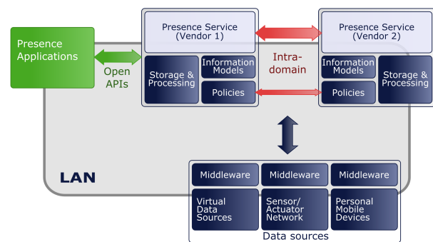
Fig. 4. Intra-domain federation
