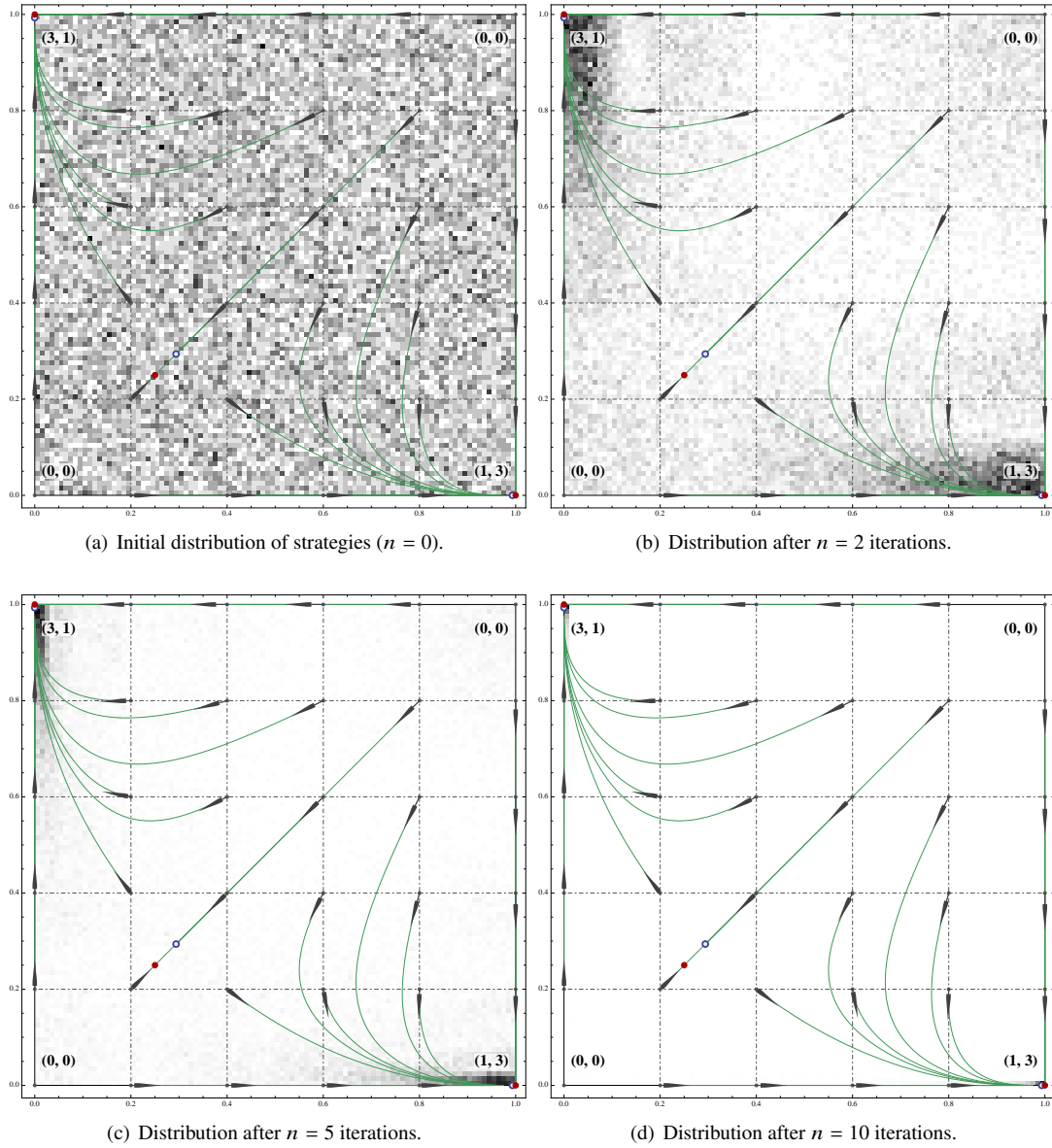
Figure 2: Snapshots of the evolution of of Algorithm 2. In our simulations, we drew 10^4 random initial strategies in the potential game of Fig. 1 and, for each strategy allocation, we ran the Boltzmann variant of Algorithm 2 with learning temperature T = 0.2 and step sequence \gamma_n = 1/(5 + n^{0.6}) . In each figure, the shades of gray represent the normalized density of states at each point of the game's strategy space and we also drew the phase portraits of the underlying mean dynamics (ED) for convenience. We see that Algorithm 2 converges to the game's QRE (which, for T = 1/\varrho = 0.2 are very close to the game's strict equilibria) quite rapidly: after only n = 10 iterations, more than 99% of the initial strategies have converged within \varepsilon = 0.01 of the game's equilibria.
