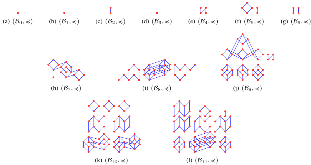
Fig. 7: Hasse diagrams of the first (\mathcal{B}_n, \preceq) posets.
