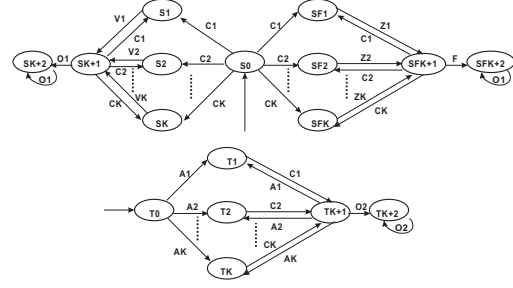
Figure 2: A system with two components G_1 (top) and G_2 (bottom) for proving undecidability of joint diagnosability.
