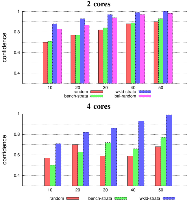
Fig. 7. Experimental degree of confidence measured with Zesto as a function of the sample size for DIP > LRU , 4 sampling methods (simple random sampling, balanced random sampling, benchmark stratification and workload stratification), using the IPCT metric.
