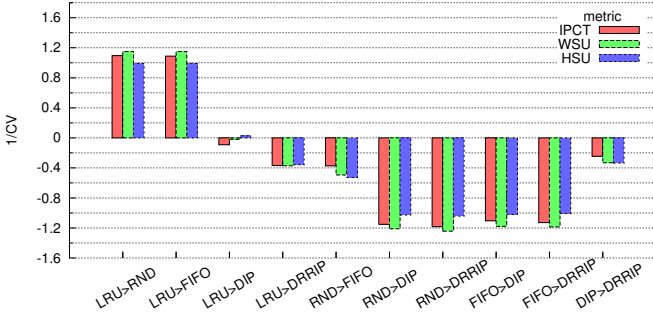
Fig. 5. Inverse of the coefficient of variation ( 1/c_v ) measured with BADCO on the full population of 12650 workloads for 4 cores.
