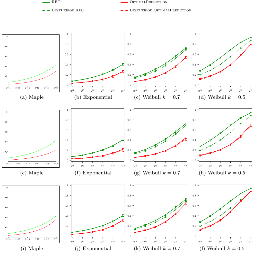
Figure 10 – Waste (y-axis) for the different heuristics as a function of the platform size (x-axis), with p = 0.82 , r = 0.85 , C_p = C (first row), C_p = 0.1C (second row), or C_p = 2C (third row) and with a trace of false predictions parametrized by a uniform distribution.
