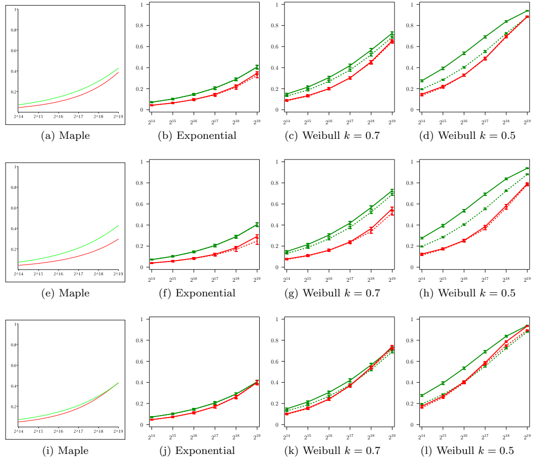
Figure 4 – Waste (y-axis) for the different heuristics as a function of the platform size (x-axis), with p = 0.4 , r = 0.7 , C_p = C (first row), C_p = 0.1C (second row), or C_p = 2C (third row) and with a trace of false predictions parametrized by a distribution identical to the distribution of the failure trace.
