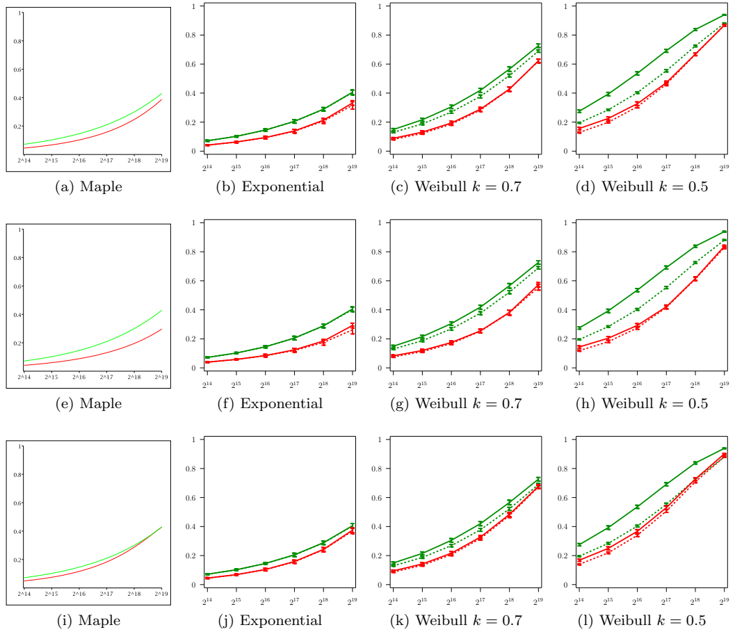
Figure 11 – Waste (y-axis) for the different heuristics as a function of the platform size (x-axis), with p = 0.4 , r = 0.7 , C_p = C (first row), C_p = 0.1C (second row), or C_p = 2C (third row) and with a trace of false predictions parametrized by a uniform distribution..
