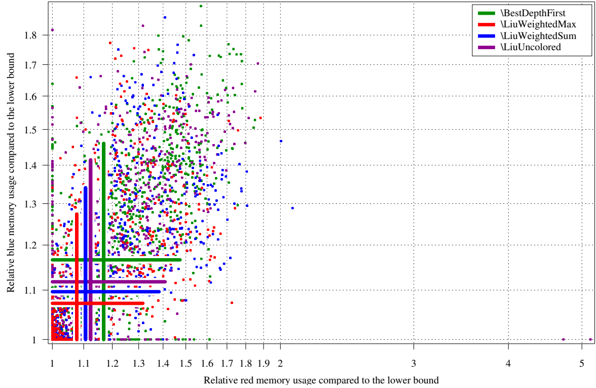
Figure 11: Distribution of each memory usage for the RANDOMWEIGHTEDREALTREES data set.
