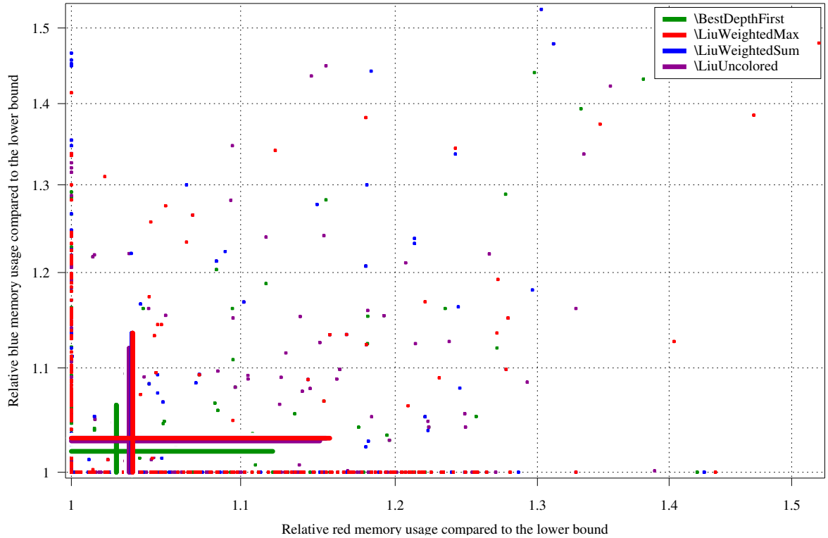
Figure 10: Distribution of each memory usage for the RANDOMCOLOREDREALTREES data set.
