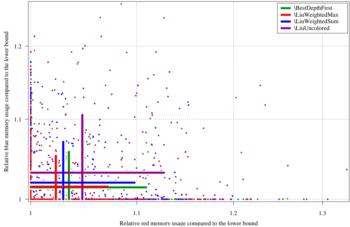
Figure 12: Distribution of each memory usage for the RANDOMTREES data set.
