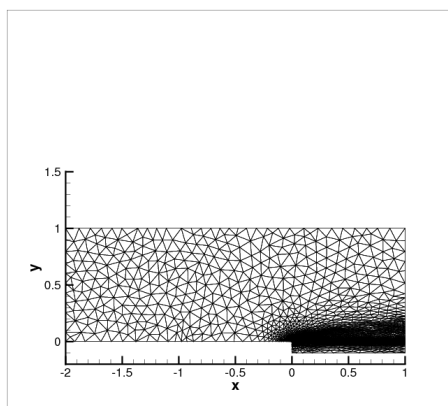
(b) Adapted mesh for the flat plate
