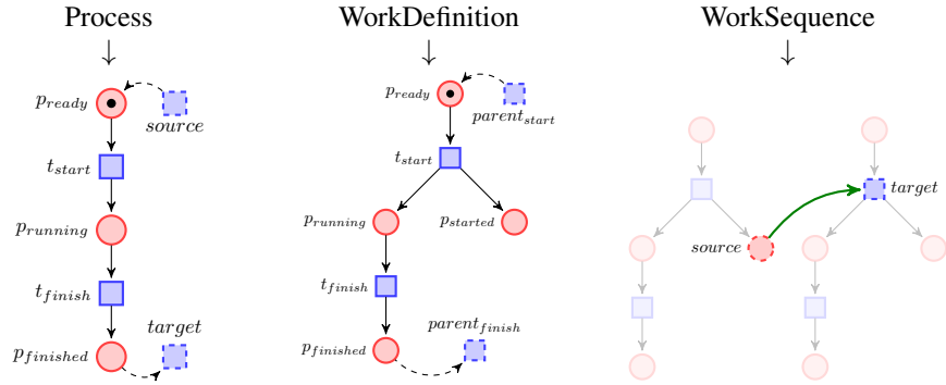
a. ProcessToPetriNet b. WorkDefinitionToPetriNet c. WorkSequenceToPetriNet
