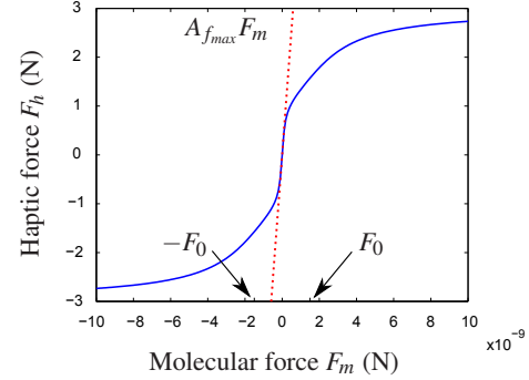
Figure 4: Profile of the force amplification using the non linear function (Equation (2)). F_{h1} = 1\text{N} , F_{h2} = 3\text{N} , F_0 = 1.5 \cdot 10^{-9}\text{N} , A_{f_{min}} = 0.64 \cdot 10^9 , A_{f_{max}} = 5.1 \cdot 10^9 .
