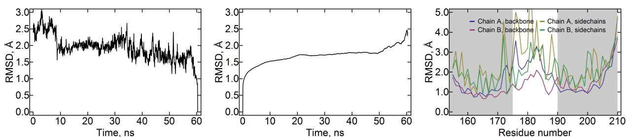
Figure S15. Structure stability of the NpHtrII HAMP2 domain as a part of the whole HAMP domain region (model 10 in Table S1).
