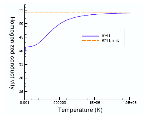
FIGURE 5.7. Asymptotic behavior of K_{11}^*
