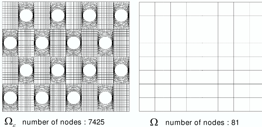
FIGURE 5.1. Initial computational meshes \Omega_\varepsilon (perforated domain) and \Omega (solid domain).
