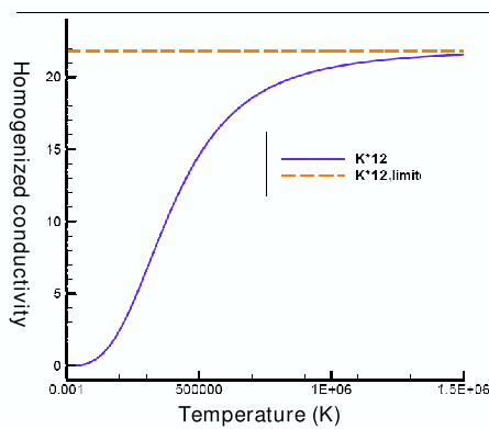
FIGURE 5.9. Asymptotic behavior of K_{12}^*
