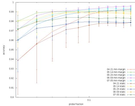
Figure 8: Accuracy comparison between the Static-Uniform and Active probe selection, curated srm-ls for the five benchmarks
