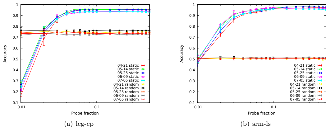
Figure 4: Accuracy for the Static-Uniform probe selection.
