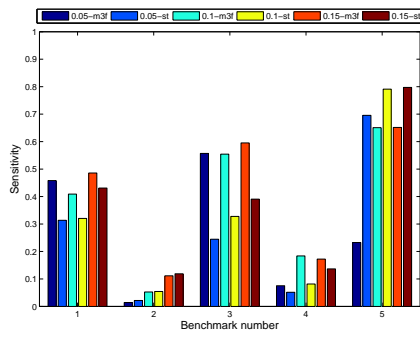
(a) Sensitivity
