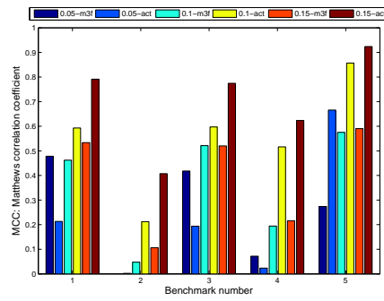
(c) MCC
