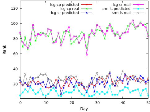
Figure 5: Rank comparison for the Static-Uniform probe selection
