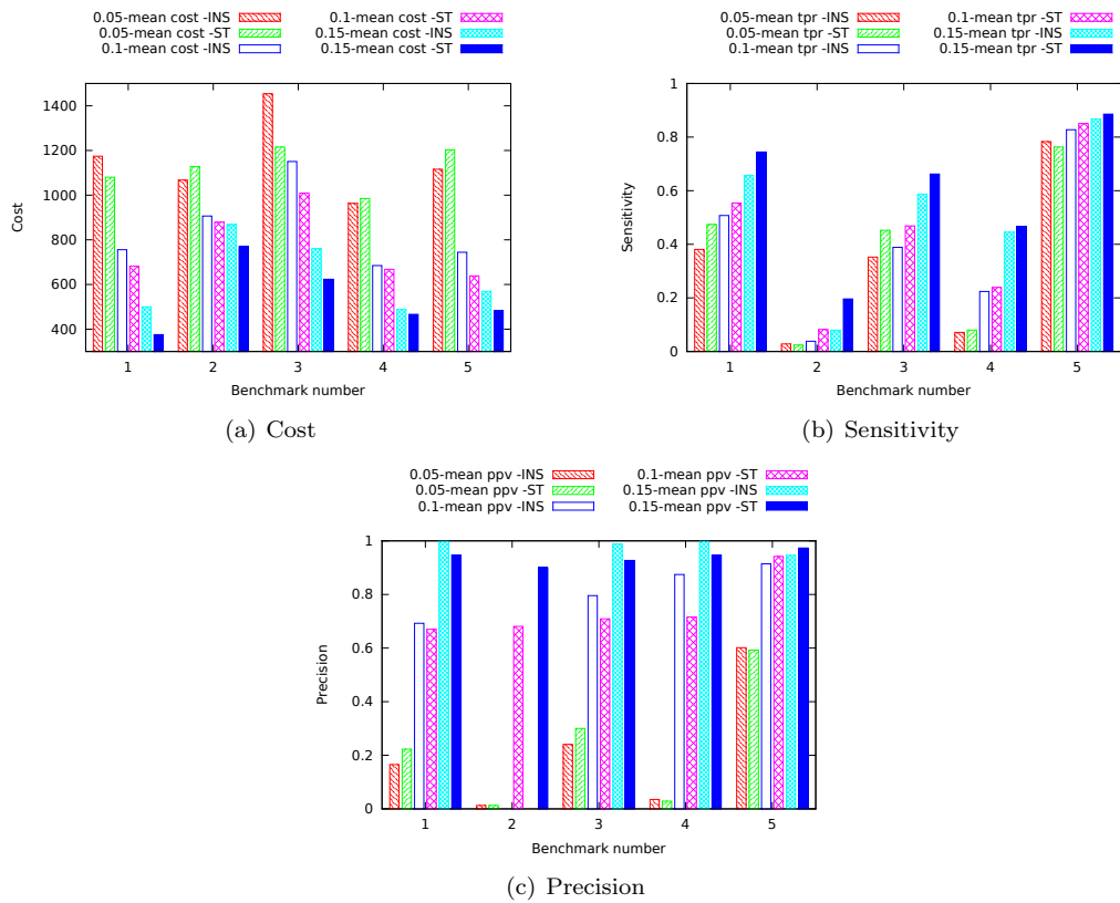
Figure 10: Cost and performance comparison between the Cost-Sensitive and Cost-Insensitive active probing, curated srm-Is for the five benchmarks.
