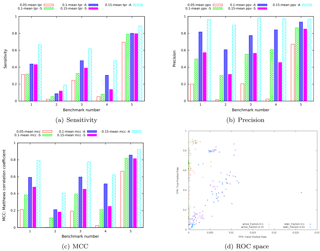
Figure 9: Performance comparison for Static-uniform and Active Probing, curated srm-ls ; , (a), (b) and (c) for the five benchmarks, (d) for all days.
