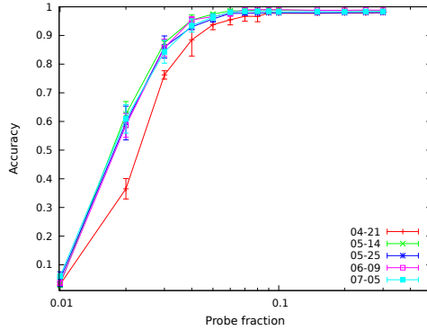
Figure 7: Accuracy for the Static-Uniform probe selection, curated srm-ls .
