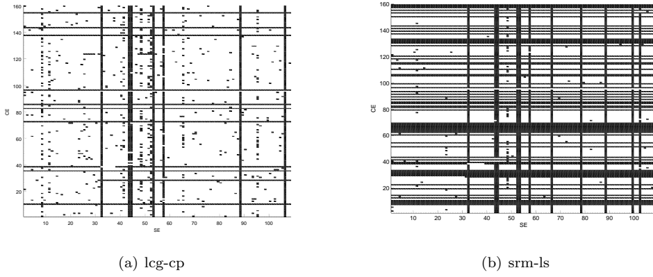
Figure 2: The CE-SE matrix. Black = FAILED, white= OK
