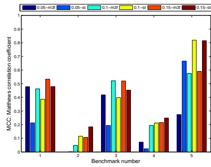
(c) MCC
