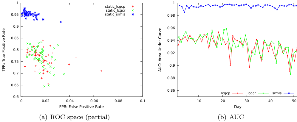
Figure 6: ROC-related metrics, Static-Uniform probe selection
