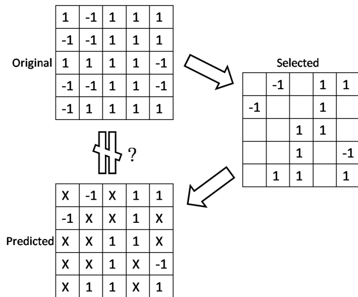
Figure 3: Illustration of matrix recovery
