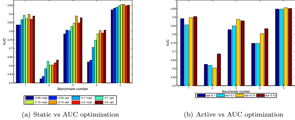
Figure 11: AUC optimization on srm-ls , with \lambda_1 = 0.5, \lambda_2 = 10 .
