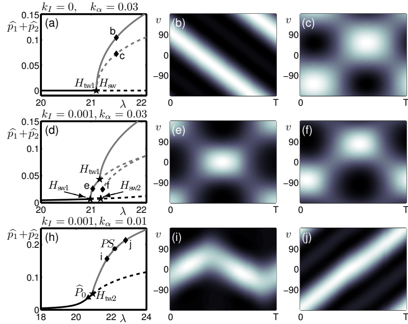
Figure 5: Changes to standing- and travelling-wave branches born in Hopf bifurcations with introduction of the stimulus. The first column shows one-parameter bifurcation diagrams in \lambda where black curves are steady-state branches and grey periodic branches; stable solution branches are solid and unstable branches are dashed. Hopf bifurcations to travelling waves are H_{tw1} and H_{tw2} , and to standing waves are H_{sw} , H_{sw1} , and H_{sw2} . Second and third columns show one period T of the solutions at corresponding points on solution branches from one-parameter diagrams.
