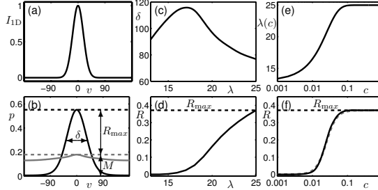
Figure 14: Model response for drifting grating stimulus and tuning of \lambda -dependence on c . (a) Stimulus profile I_{1D}(v) for a visual-field-covering drifting grating. (b) Steady state responses at \lambda = 13 (grey curve) and at \lambda = 25 (black curve); dashed horizontal lines indicate the maximum activity for these steady states. The tuning bandwidth, or tuning width at half-height, is \delta and the maximum level of activity above the spontaneous level (dashed grey line) is R . (c) Tuning width \delta of response for \lambda \in [\lambda_{\min}, \lambda_{\max}] . (d) Normalised response R for \lambda \in [\lambda_{\min}, \lambda_{\max}] . (e) Variation of \lambda with respect to c . (f) Contrast response curve with \lambda varying as in (e) (black) and the Naka-Rushton function with parameters as described in the text (dashed grey).
