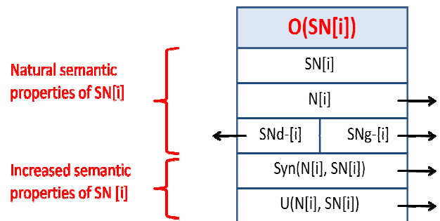
Figure 8: Structure of the NP ontology.
