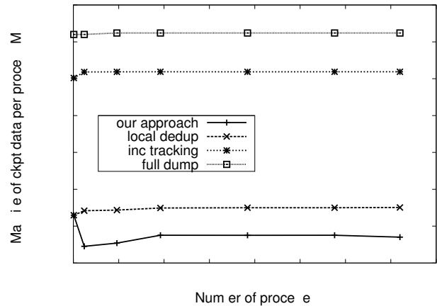
(b) Maximal amount of checkpointing data saved per process (lower is better)
