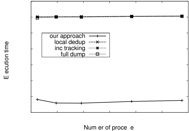
(b) Total time for all benchmarking processes to finish execution
