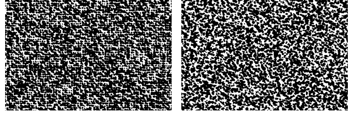
(a) Grid placement of stipples. (b) After random perturbation.
