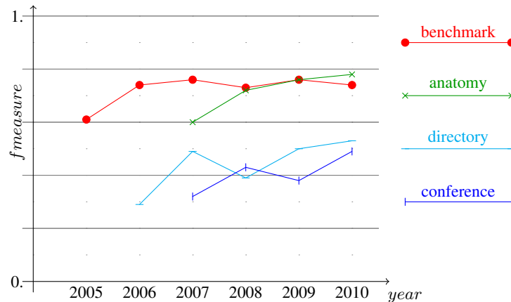
Fig. 6. Evolution of the average f-measure in different datasets.
