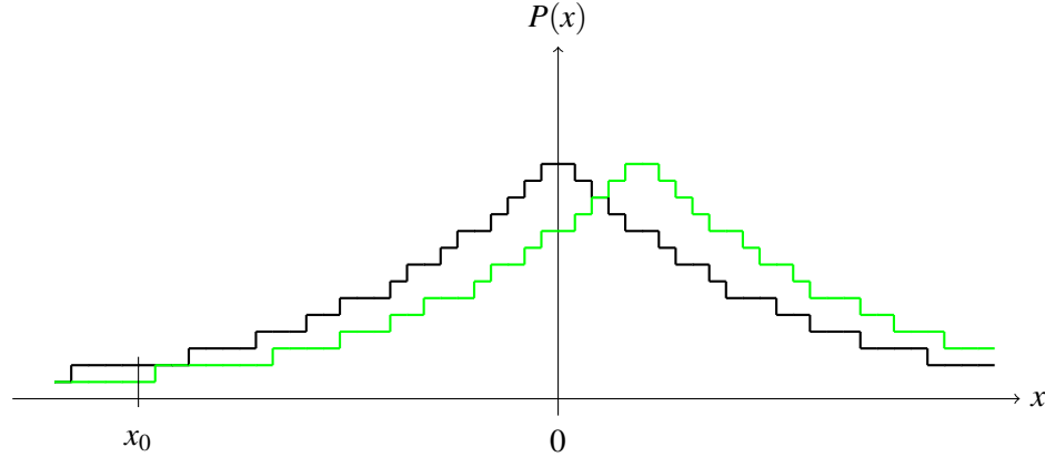
Figure 2: The probability distributions of Laplace noises generated from a discretized uniform generator
