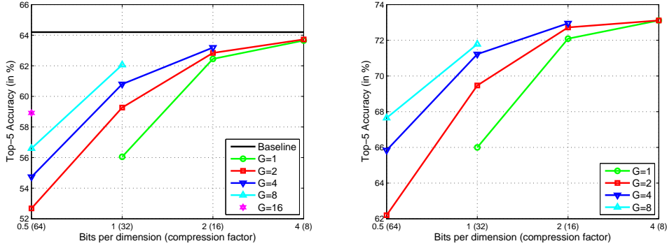
Figure 8: Compression results on ILSVRC 2010 with 4K-dim FVs (left) and 64K-dim FVs when varying the number of bits per dimension b and the sub-vector dimensionality G .
