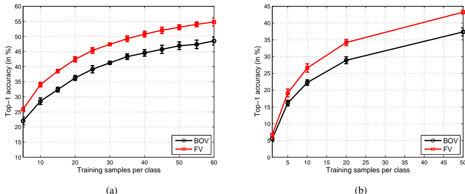
Figure 7: Comparison of the soft-BoV and the FV on Caltech256 (left) and SUN 397 (right) as a function of the number of training samples. We only use SIFT descriptors and report the mean and 3 times the average deviation.
