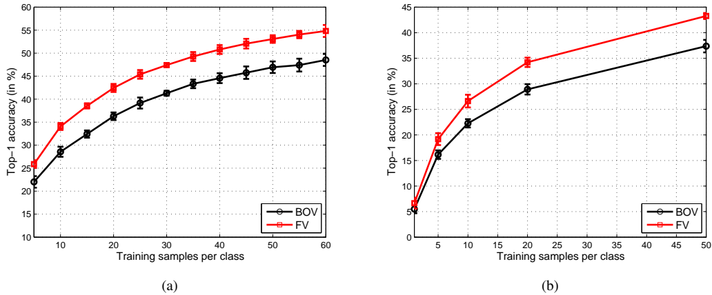
Figure 2: Comparison of the soft-BoV and the FV on Caltech256 (left) and SUN 397 (right) as a function of the number of training samples. We only use SIFT descriptors and report the mean and 3 times the average deviation.
