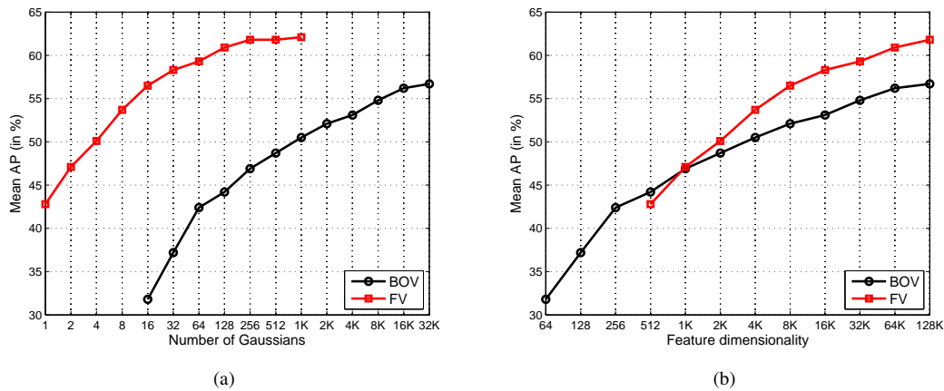
Figure 1: Accuracy of the soft-BoV and the FV as a function of the number of Gaussians (left) and feature dimensionality (right) on PASCAL VOC 2007 with SIFT descriptors only.
