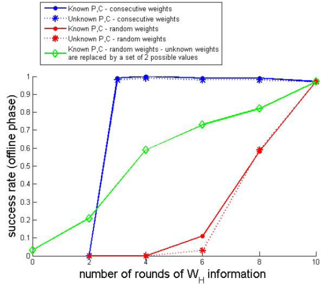
Fig. 23 Success rate of the attacks against an unprotected implementation of the AES in function of the amount of exploited leakages. One round of side-channel information is equivalent to 84 known Hamming weights
