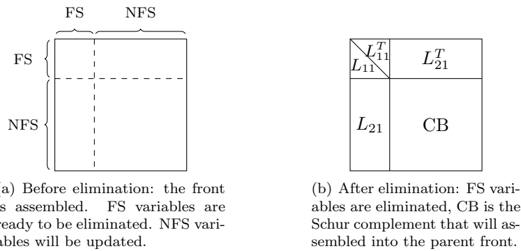
FIGURE 2.3. Structure of a front F .
