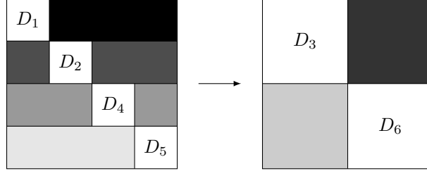
FIGURE 3.3. Structure of a HSS matrix and its basic construction scheme
