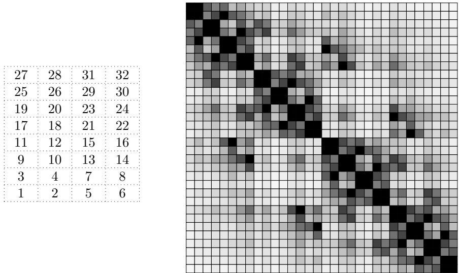
(a) Numbering scheme of the graph associated with the Schur complement. The numbers give the ordering of the 32 blocks of 32 \times 16 = 512 variables within the BLR structure. Any other numbering of the clusters would give equivalent results.
