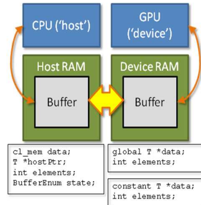
Fig. 4: Data elements on CPU and GPU
