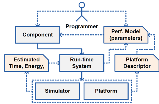
Fig. 5: Overview of performance modeling in PEPPHER. Performance models are provided by the component developer or automatically generated by the run-time system.
