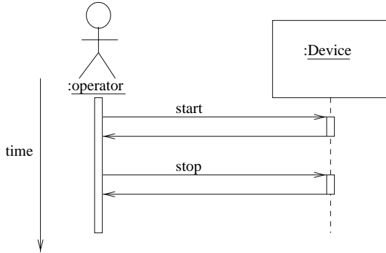
Figure 5. UML sequence diagram
