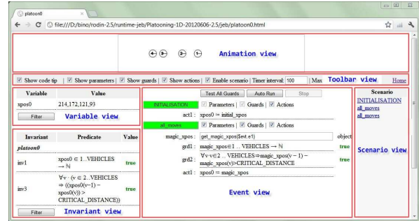
Figure 2: Simulation window
