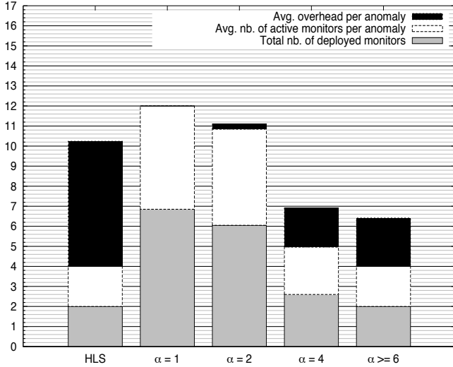
(a) Localization cost
