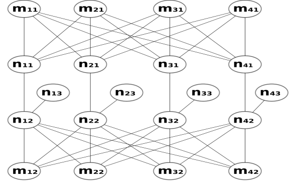
Fig. 2: Example of a graph constructed out of a facility location instance with four facility locations and four clients
