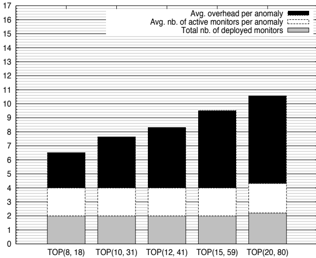
Fig. 4: Localization cost of the heuristic solutions, \alpha \gg \beta
