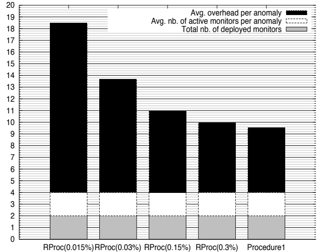
Fig. 5: Numerical results for TOP(15, 59). Impact of the number and the quality of candidate monitoring paths on the quality of the localization solution. RProc means random procedure.
