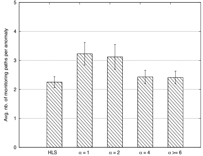
(b) Average number of monitoring paths per anomaly
