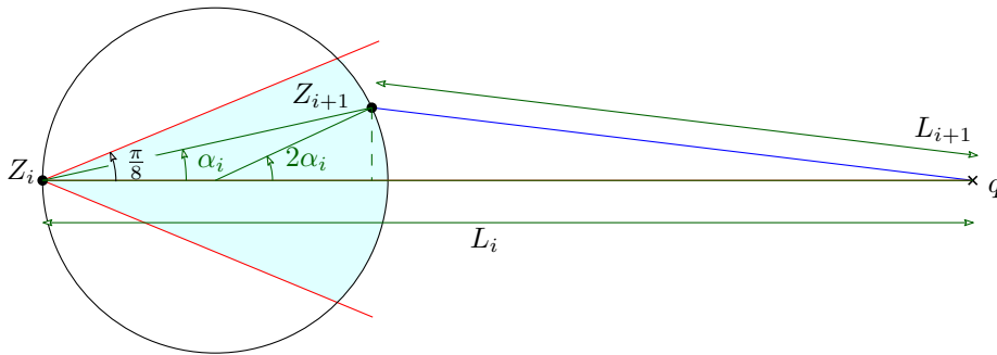
Figure 7: For the angle to be smaller than \alpha given R \in [r, r + \epsilon] , the stopper must fall within the dark shaded region
