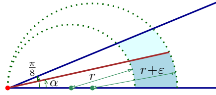
Figure 7: For the angle to be smaller than \alpha given R \in [r, r + \epsilon] , the stopper must fall within the dark shaded region
