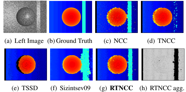
Figure 2. Synthetic dataset of [4]. Frame 6, noise level \sigma = 0.5 . Disparity maps.
