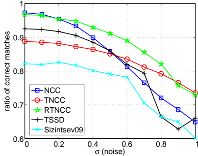
Figure 1. Quantitative evaluation.
