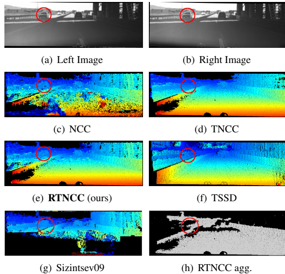
Figure 3. DAGM Exposure Challenge dataset. Disparity maps.
