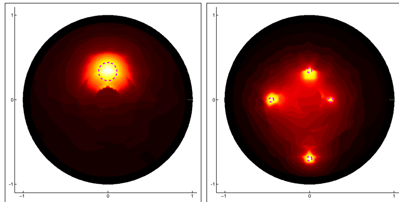
Fig. 8. Coloring of C(\xi) . Left: i2UN, \gamma = 5 \cdot 10^{-2} . Right: i2US, \gamma = 10^{-2} .
