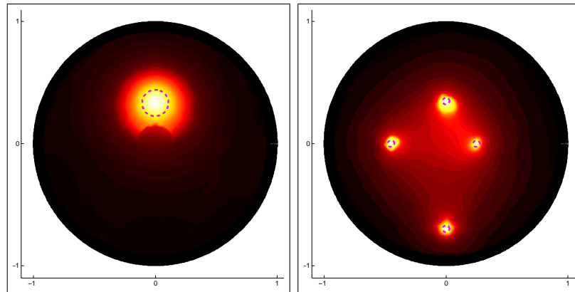
Fig. 7. Coloring of C(\xi) . Left: i1UN, \gamma = 5 \cdot 10^{-2} . Right: i1US, \gamma = 5 \cdot 10^{-3} .
