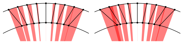
Fig. 4 Visualization of the relationship between \phi_j (inner points) and \theta_j (outer points) for the left and right cameras. The connecting lines would be purely radial if all \{\theta_j, \phi_j\} pairs were equal. The area of each translucent sector is proportional to the corresponding angular discrepancy |\phi_j - \theta_j| .
