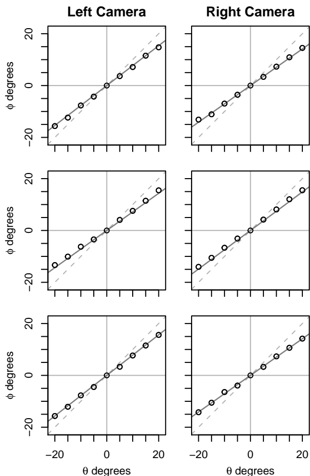
Fig. 8 Homography-angles \phi_j plotted as a function of the motor-angles \theta_j . Three trials are shown (rows) for each camera (columns). The least-squares regression model is drawn through the data points. It can be seen that the homography/motor relationship is approximately linear, with a slope \eta < 1 . The dashed line, for comparison, has unit slope.
