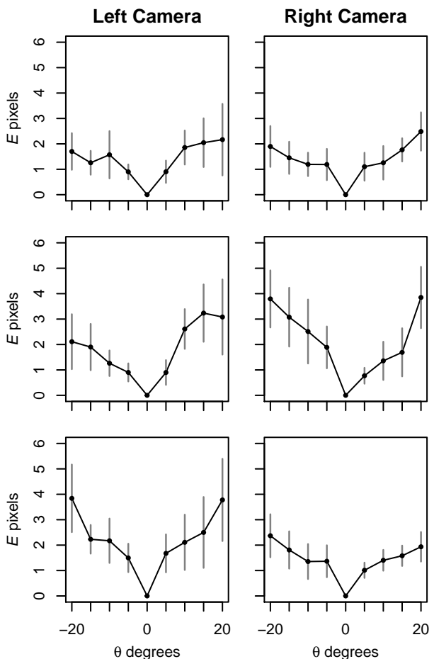
Fig. 9 Symmetric transfer error (16) as a function of the homography angle \theta_j (in images of size 1024 \times 768 ). Three trials are shown (rows) for each camera (columns), as in Fig. 8. The vertical bars indicate the spread \pm\sigma of the errors around the corresponding mean. Note that \mathbf{H}_0 = \mathbf{I} , by definition, and so there is no error at \theta = 0 .
