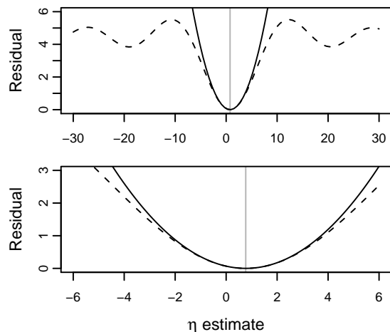
Fig. 5 Comparison of the angular (dashed) and Euclidean (solid) metrics (9), on the actual data-set. The upper plot shows periodic form of the angular error. The global minimum is well-approximated by a parabola, as in (10). The least-squares estimate (12) is the minimum of the parabola, indicated by the vertical line. For the present data, the difference between the two metrics is insignificant. The lower plot shows a magnified view.
