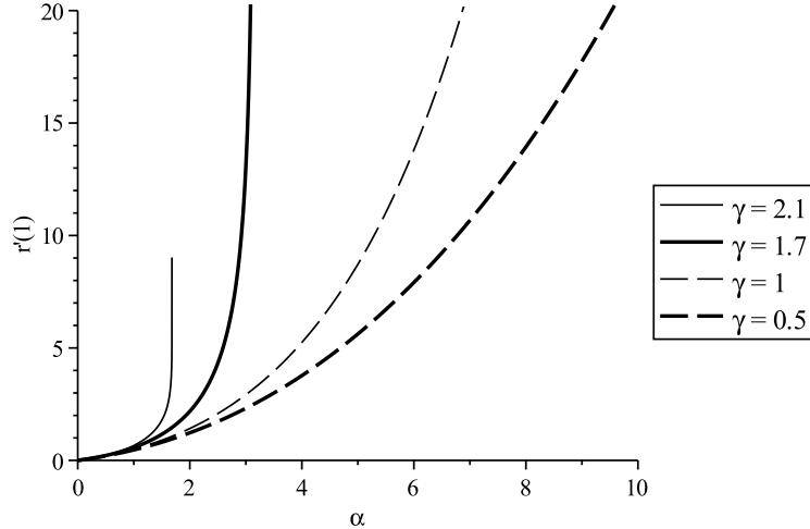
Figure 1: Expected score of POIs per player r'(1) as a function of the visit rate \alpha . The parameters \lambda = \mu = 3 remain fixed.
